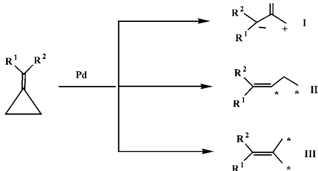
Scheme 1. Three Reaction Patterns of MCPs
